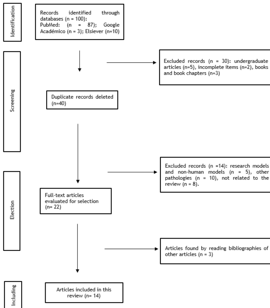
Figure 1. PRISMA flow diagram showing the article selection process
